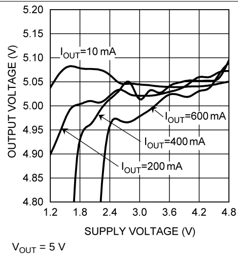
图 7. Output Voltage vs Supply Voltage
