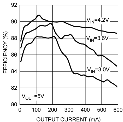
图 10. Efficiency vs Output Current
