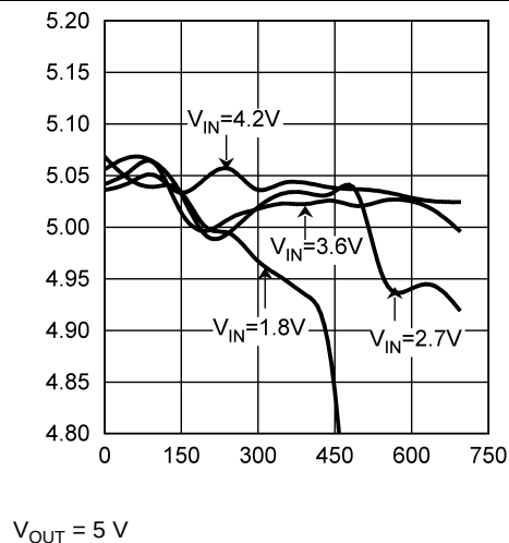
图 11. Output Voltage vs Output Current
