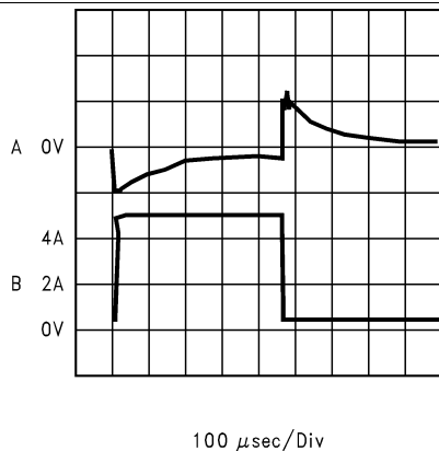
Load Transient Response for Continuous Mode V_{IN} = 20\text{ V} , V_{OUT} = 5\text{ V} , L = 10\text{ }\mu\text{H} , C_{OUT} = 400\text{ }\mu\text{F} , C_{OUT}ESR = 13\text{ m}\Omega A. Output voltage, 100 mV/div, AC-coupled B. Load current: 500-mA to 5-A load pulse
