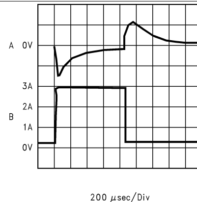
Load Transient Response for Discontinuous Mode V_{IN} = 20\text{ V} , V_{OUT} = 5\text{ V} , L = 10\text{ }\mu\text{H} , C_{OUT} = 400\text{ }\mu\text{F} , C_{OUT}ESR = 13\text{ m}\Omega A. Output voltage, 100 mV/div, AC-coupled B. Load current: 200-mA to 3-A load pulse
