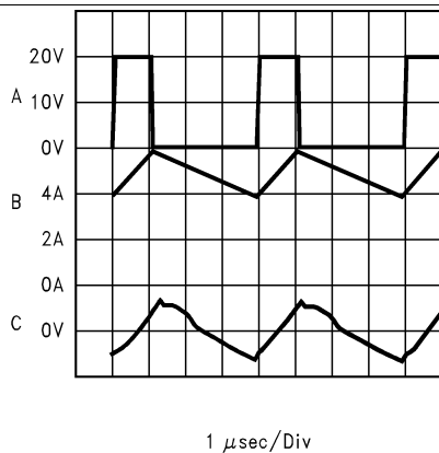
Continuous Mode Switching Waveforms V_{IN} = 20\text{ V} , V_{OUT} = 5\text{ V} , I_{LOAD} = 5\text{ A} , L = 10\text{ }\mu\text{H} , C_{OUT} = 400\text{ }\mu\text{F} , C_{OUT}ESR = 13\text{ m}\Omega A. V_{SW} pin voltage, 10 V/div B. Inductor current, 2 A/div C. Output ripple voltage, 20 mV/div AC-coupled
