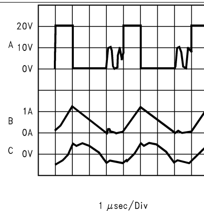
Discontinuous Mode Switching Waveforms V_{IN} = 20\text{ V} , V_{OUT} = 5\text{ V} , I_{LOAD} = 500\text{ mA} , L = 10\text{ }\mu\text{H} , C_{OUT} = 400\text{ }\mu\text{F} , C_{OUT}ESR = 13\text{ m}\Omega A. V_{SW} pin voltage, 10 V/div B. Inductor current, 1 A/div C. Output ripple voltage, 20 mV/div AC-coupled
