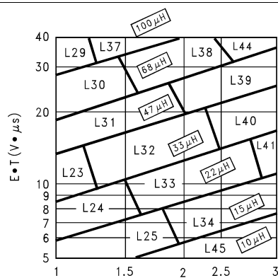
Figure 20. LM2676-ADJ
