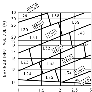
Figure 19. LM2676-12
