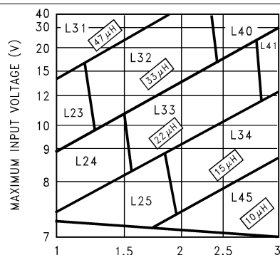
Figure 18. LM2676-5
