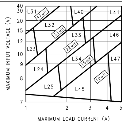
Figure 18. LM2678-5
