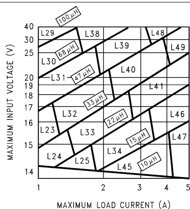
Figure 19. LM2678-12
