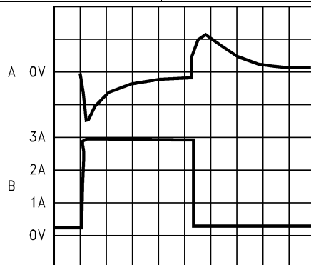
200 \mu\text{sec}/\text{Div} Load Transient Response for Discontinuous Mode V_{\text{IN}} = 20\text{ V} , V_{\text{OUT}} = 5\text{ V} , L = 10\text{ }\mu\text{H} , C_{\text{OUT}} = 400\text{ }\mu\text{F} , C_{\text{OUTESR}} = 13\text{ m}\Omega A: Output Voltage, 100 mV/div, AC-Coupled B: Load Current: 200-mA to 3-A Load Pulse
