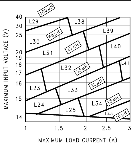
Figure 19. LM2670 – 12 V
