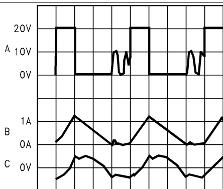
1 \mu\text{sec}/\text{Div} Discontinuous Mode Switching Waveforms V_{\text{IN}} = 20\text{ V} , V_{\text{OUT}} = 5\text{ V} , I_{\text{LOAD}} = 500\text{ mA} L = 10\text{ }\mu\text{H} , C_{\text{OUT}} = 400\text{ }\mu\text{F} , C_{\text{OUTESR}} = 13\text{ m}\Omega A: V_{\text{SW}} Pin Voltage, 10 V/div B: Inductor Current, 1 A/div C: Output Ripple Voltage, 20 mV/div AC-Coupled
