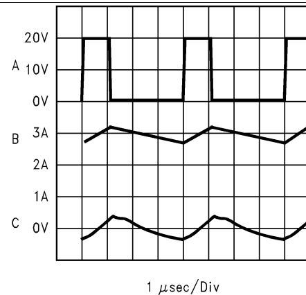
Figure 10. Switching Frequency
