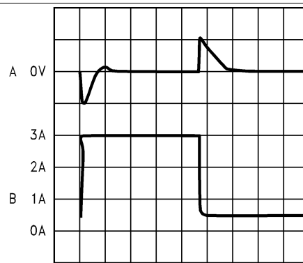
100 \mu\text{sec}/\text{Div} Load Transient Response for Continuous Mode V_{\text{IN}} = 20\text{ V} , V_{\text{OUT}} = 5\text{ V} L = 33\text{ }\mu\text{H} , C_{\text{OUT}} = 200\text{ }\mu\text{F} , C_{\text{OUTESR}} = 26\text{ m}\Omega A: Output Voltage, 100 mV/div, AC-Coupled B: Load Current: 500-mA to 3-A Load Pulse
