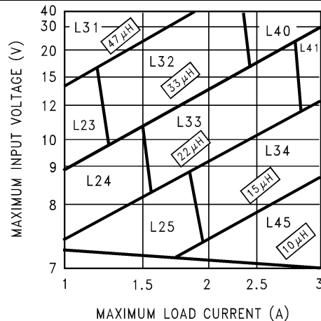
Figure 18. LM2670 – 5 V
