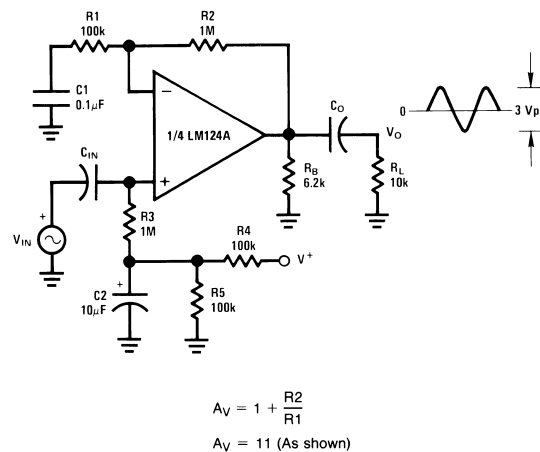
Figure 37. AC Coupled Non-Inverting Amplifier
