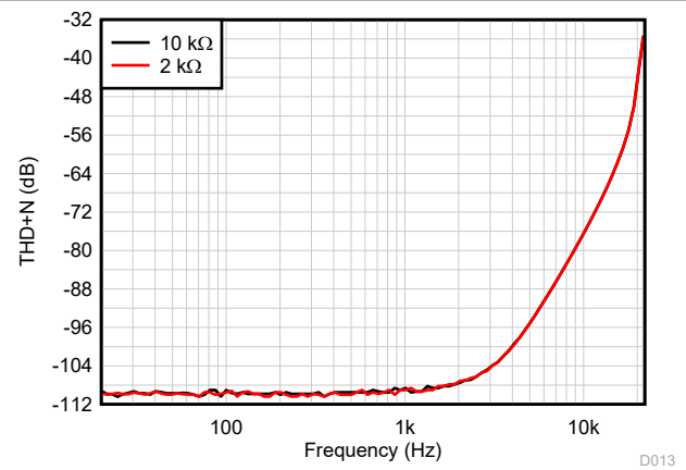
图 6-18. THD+N Ratio vs Frequency, G = 1 G = 1 , f = 1\text{ kHz} , BW = 80\text{ kHz} , V_{OUT} = 10\text{ V}_{PP} , R_L connected to V_-
