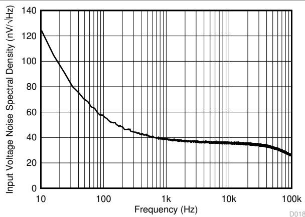
图 6-12. Input Voltage Noise Spectral Density
