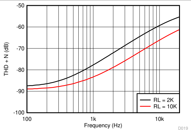
图 6-13. THD + N vs Frequency
