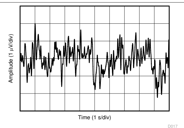
图 6-11. 0.1-Hz to 10-Hz Integrated Voltage Noise
