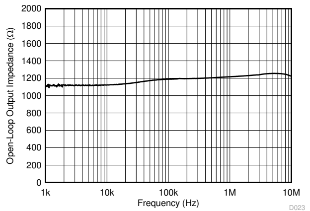
图 6-17. Open-Loop Output Impedance vs Frequency
