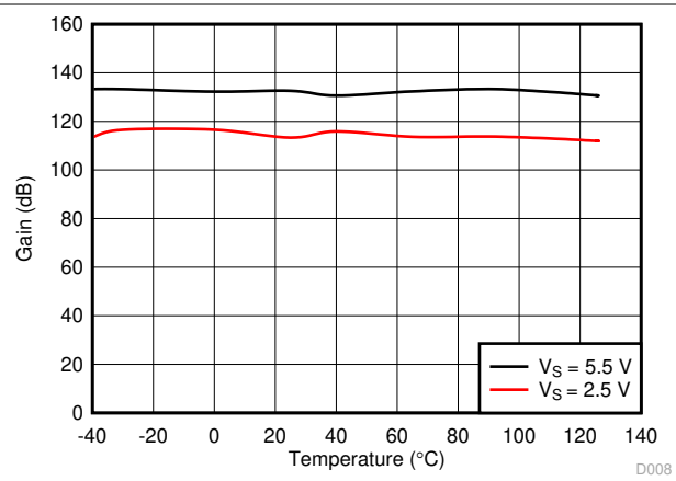
图 6-2. Open-Loop Gain vs Temperature
