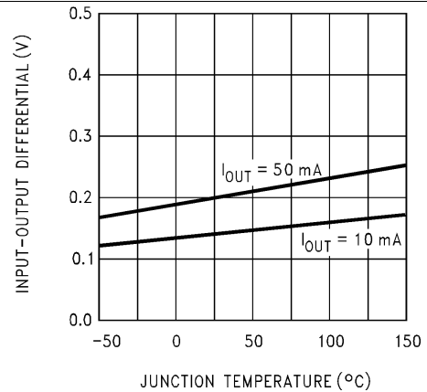
Figure 2. Dropout Voltage
