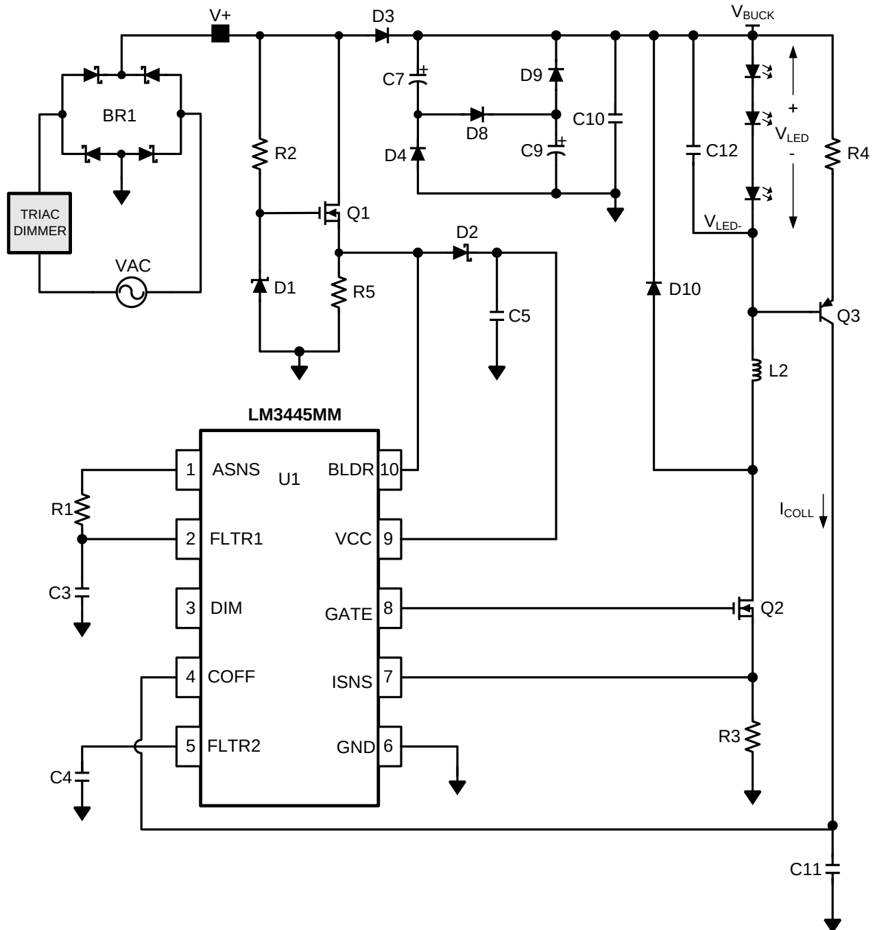
Figure 11. LM3445 Schematic
