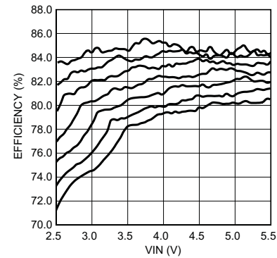
L = 4.7\text{ }\mu\text{H} 20\text{ mA/String} Top To Bottom: 1x4, 1x5, 1x6, 1x7, 1x8, 1x9, 1x10 (LEDs)
