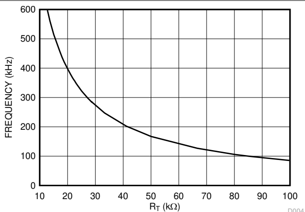
图 6-3. Oscillator Frequency
