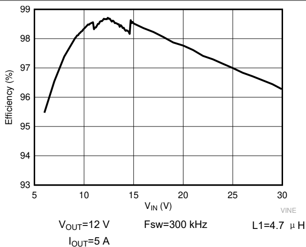
图 6-1. Efficiency vs V_{IN}
