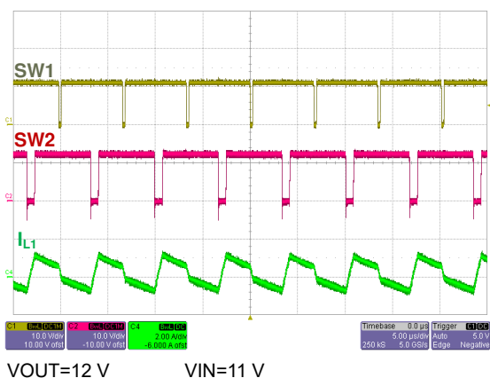
图 6-11. Forced CCM Operation (Buck-Boost)
