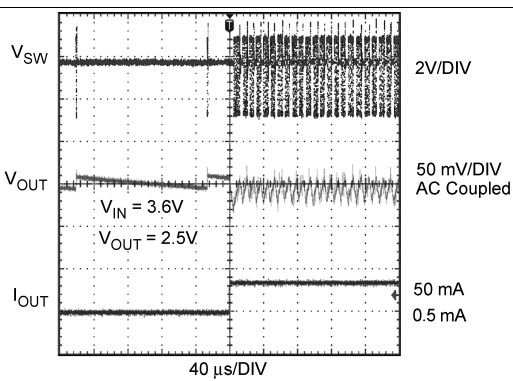
Figure 21. Load Transient Response
