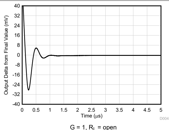
图 6-32. Large-Signal Step Response (Falling)
