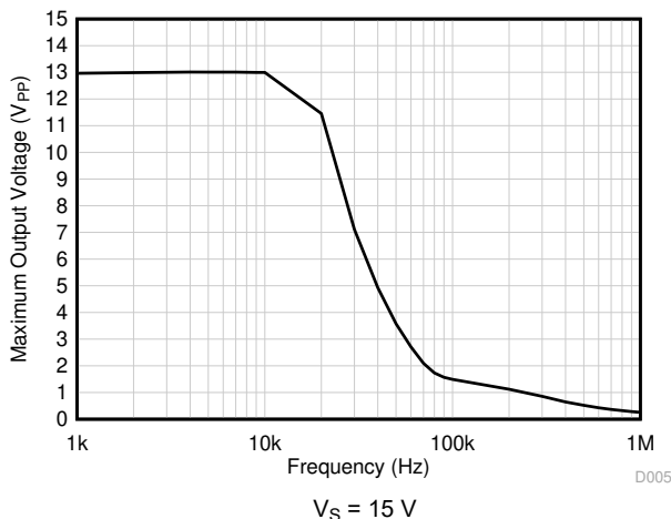
图 6-36. Maximum Output Voltage vs Frequency
