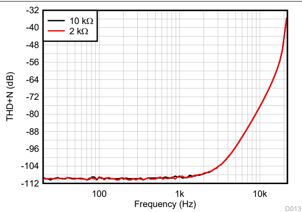
G = 1 , f = 1\text{ kHz} , BW = 80\text{ kHz} , V_{OUT} = 10\text{ V}_{PP} , R_L connected to V_- 图 6-18. THD+N Ratio vs Frequency, G = 1
