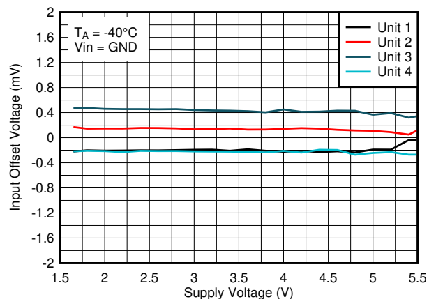
Figure 6-30. Offset Voltage vs. Supply Voltage at -40°C, VIN=0V
