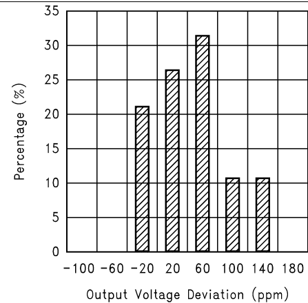
Figure 14. Long-Term Drift
