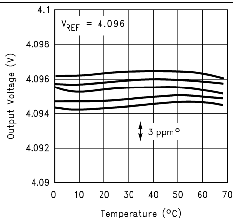
Figure 29. Typical Temperature Coefficient (Sample of 5 Parts)
