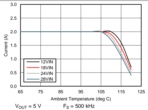
Figure 62. Derating Curve
