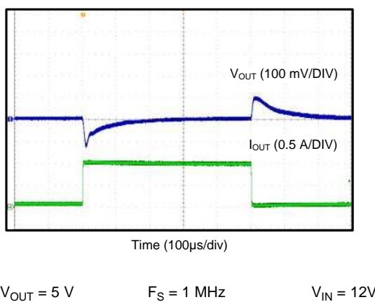
Figure 61. Load Transient 0.1A to 1A
