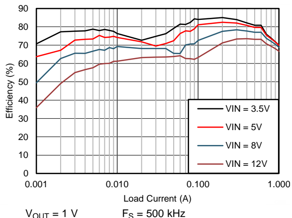
Figure 48. Efficiency
