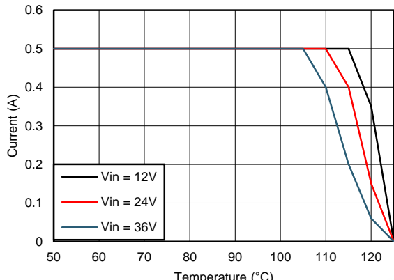
Figure 90. Derating Curve with R_{\theta JA} = 20^\circ\text{C/W}
