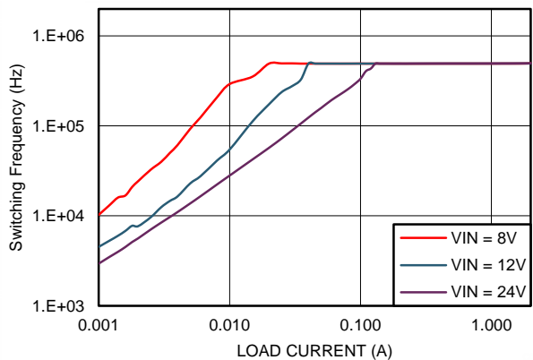
Figure 93. Switching Frequency vs I_{OUT} in PFM Operation
