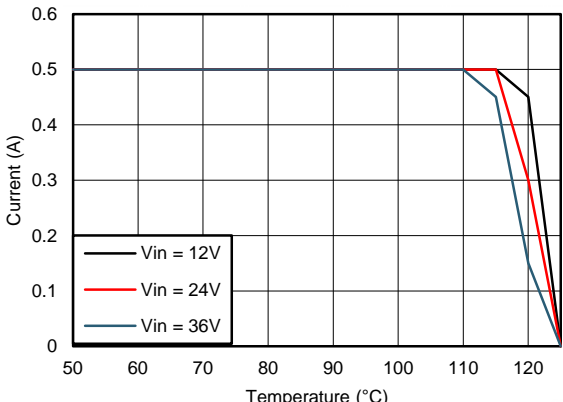
Figure 89. Derating Curve with R_{\theta JA} = 20^\circ\text{C/W}
