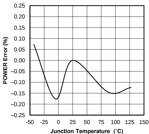
Figure 10. PIN Measurement Error ( V_{IN\_K} - SENSE = 22\text{ mV} )
