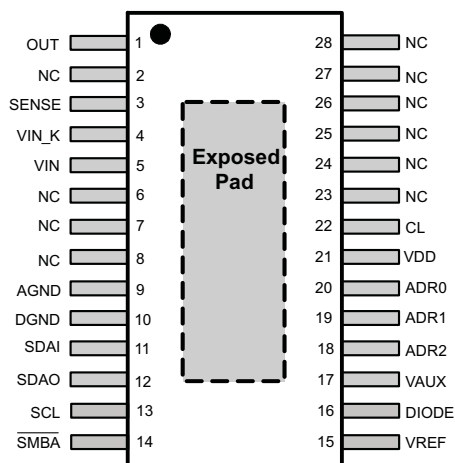
HTSSOP Package 28 Pin (Top View)
