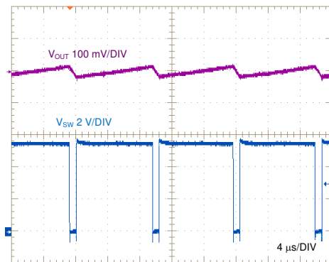
图 8-5. SW Node and Output Ripple Voltage, No Load
