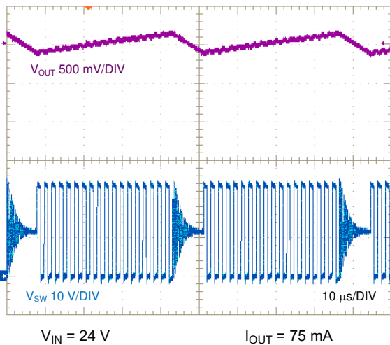
图 8-24. SW Node and Output Ripple Voltage, Full Load
