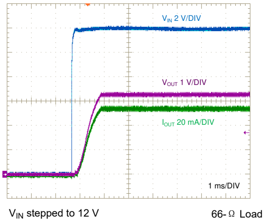
图 8-17. Start-Up, Full Load
