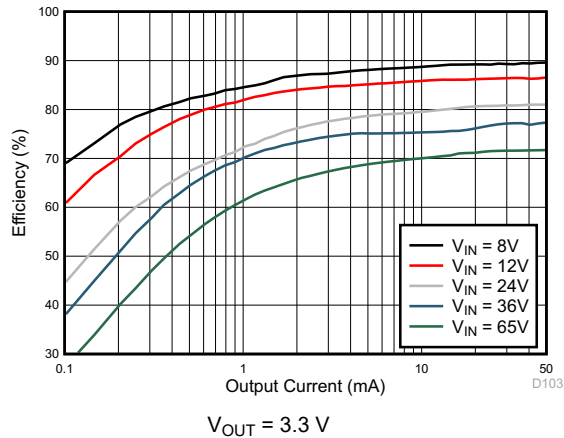
图 8-15. Efficiency
