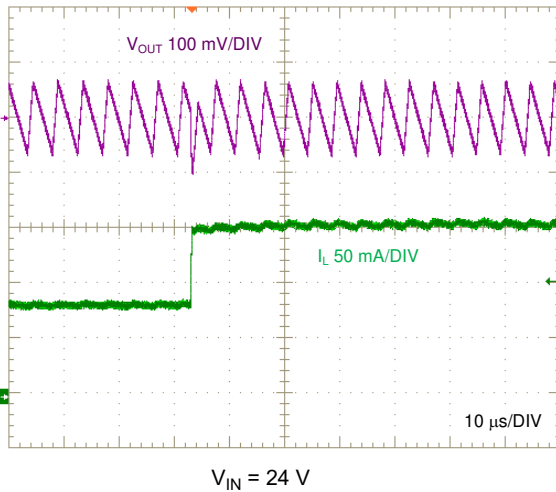
图 8-12. Load Transient, 50 mA to 150 mA, 1 A/ \mu s
