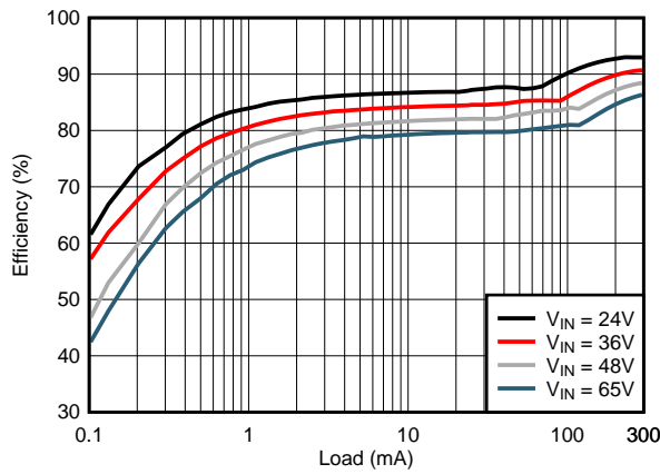
图 85. Converter Efficiency
