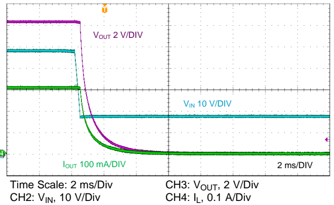
图 88. Shutdown Waveforms
