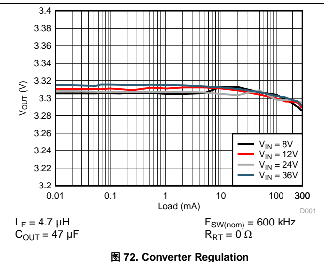
图 72. Converter Regulation
