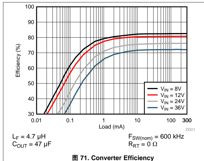
图 71. Converter Efficiency
