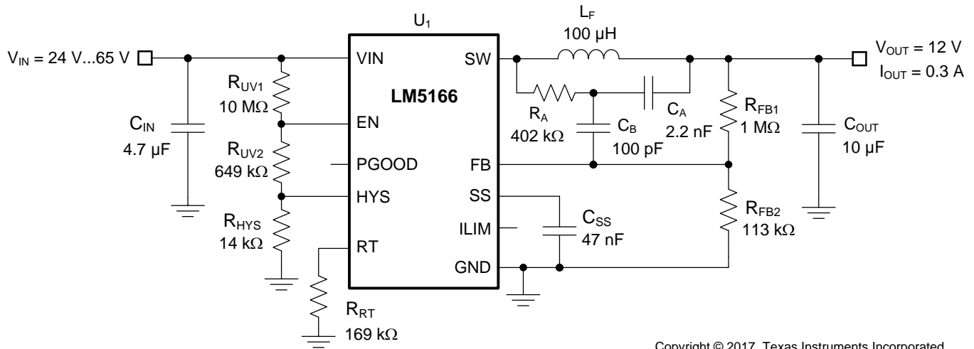
图 84. Schematic for Design 5 With V_{OUT} = 12\text{ V} , I_{OUT(max)} = 300\text{ mA} , F_{SW(nom)} = 400\text{ kHz}
