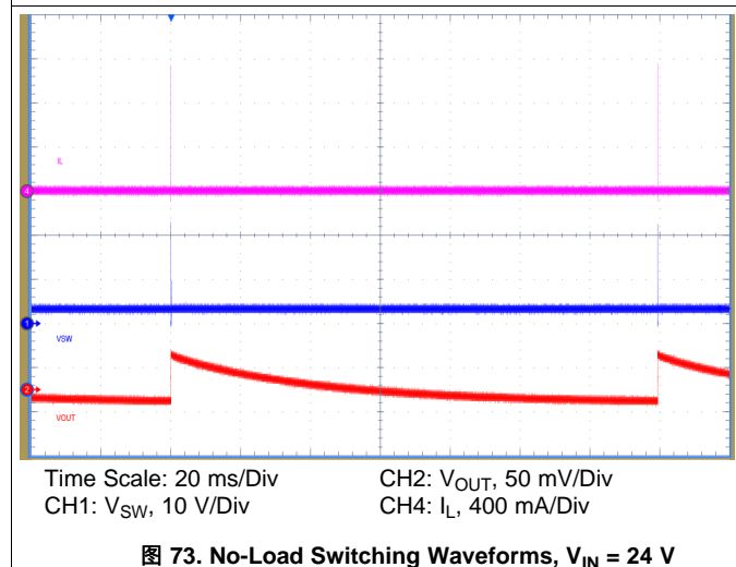
图 73. No-Load Switching Waveforms, V_{IN} = 24\text{ V}
