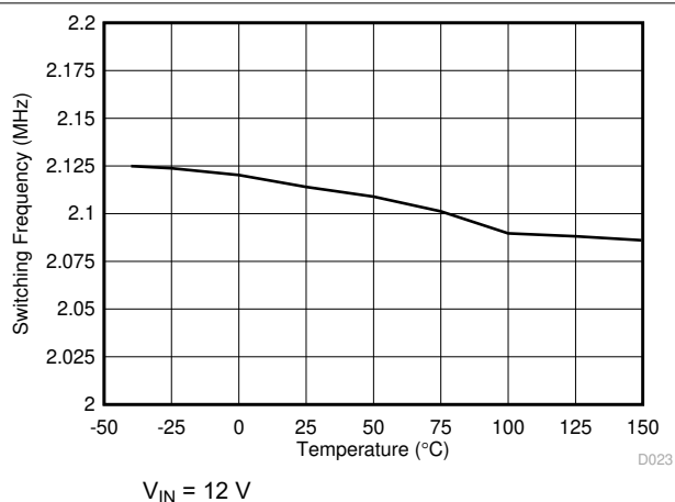
图 7-2. Switching Frequency vs Temperature
