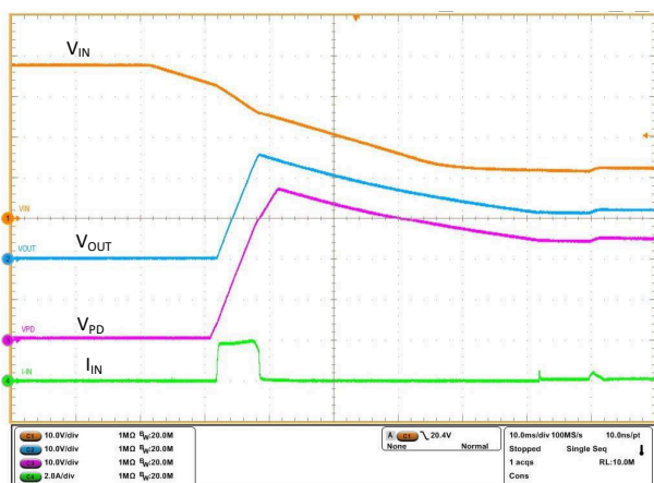
图 9-17. Overvoltage Recovery
