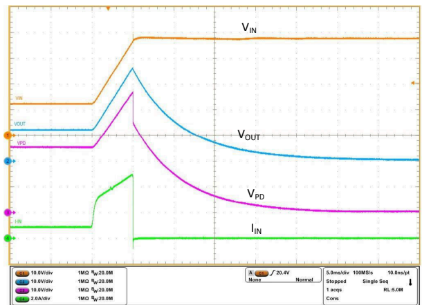
图 9-16. Overvoltage Protection
