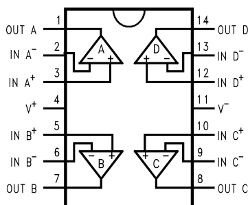
Figure 2. 14-Pin TSSOP/SOIC
