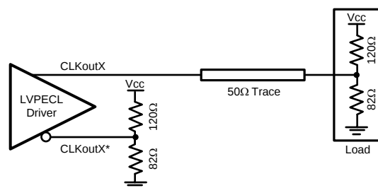
Figure 16. Single-Ended LVPECL Operation, DC Coupling, Thevenin Equivalent
