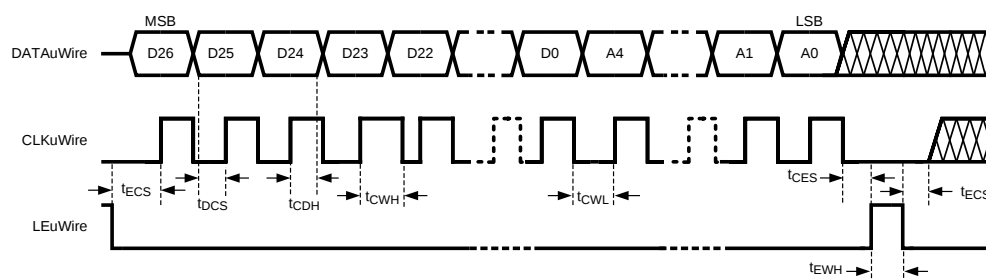
Figure 1. MICROWIRE Input Timing Diagram
