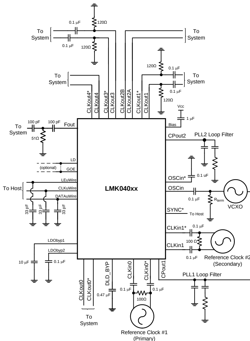
Figure 13. Typical Application
