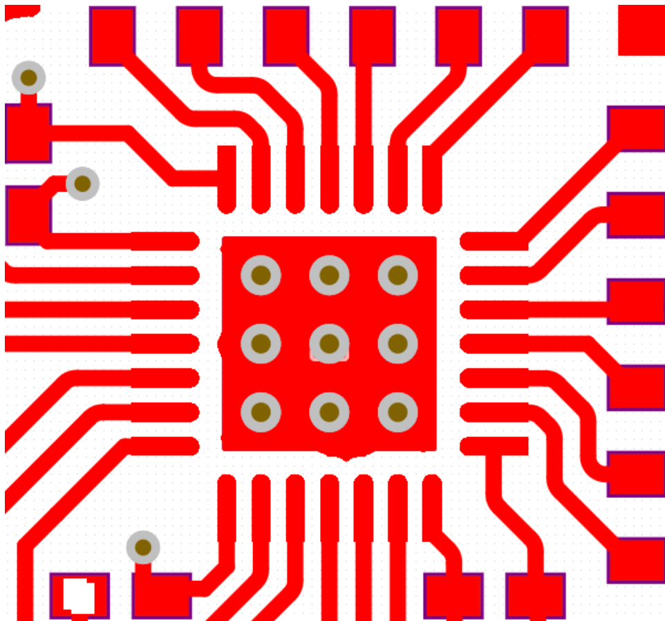
图 11-1. Recommended PCB Layout, Top Layer
