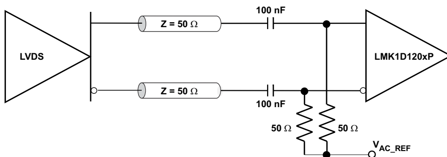
图 8-4. LVDS Clock Driver Connected to LMK1D1204P Input (AC-Coupled)
