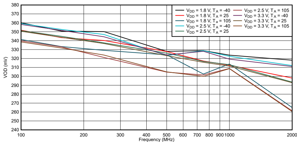
图 6-2. LMK1D1204P VOD vs. Frequency
