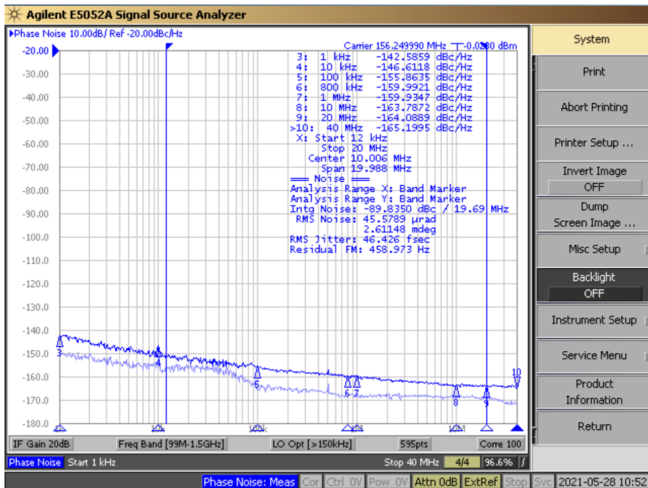
图 9-3. LMK1D1204P Output Phase Noise, 156.25 MHz, 46.4-fs RMS (12 kHz to 20 MHz)
