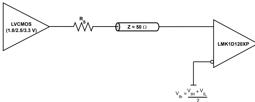
图 8-6. 1.8-V/2.5-V/3.3-V LVCMOS Clock Driver Connected to LMK1D1204P Input
