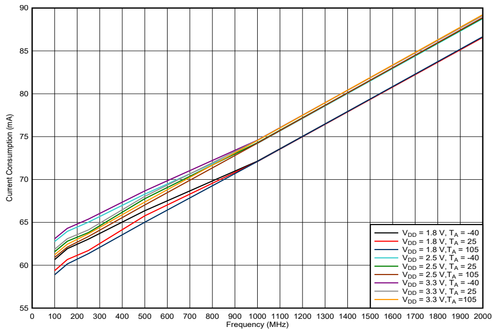
图 6-1. LMK1D1204P Current Consumption vs. Frequency
