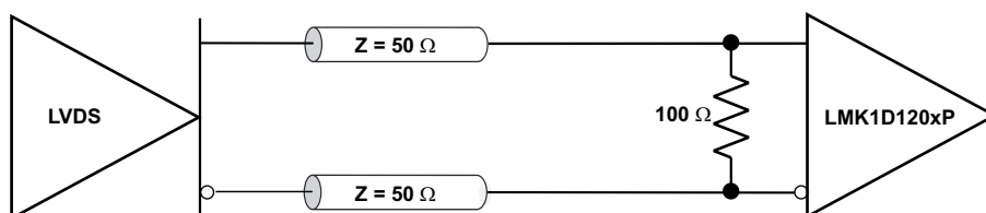
图 8-3. LVDS Clock Driver Connected to LMK1D1204P Input (DC-Coupled)
