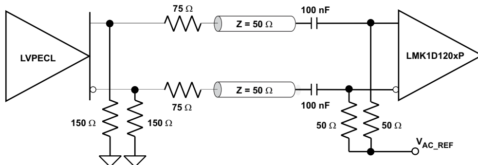
图 8-5. LVPECL Clock Driver Connected to LMK1D1204P Input
