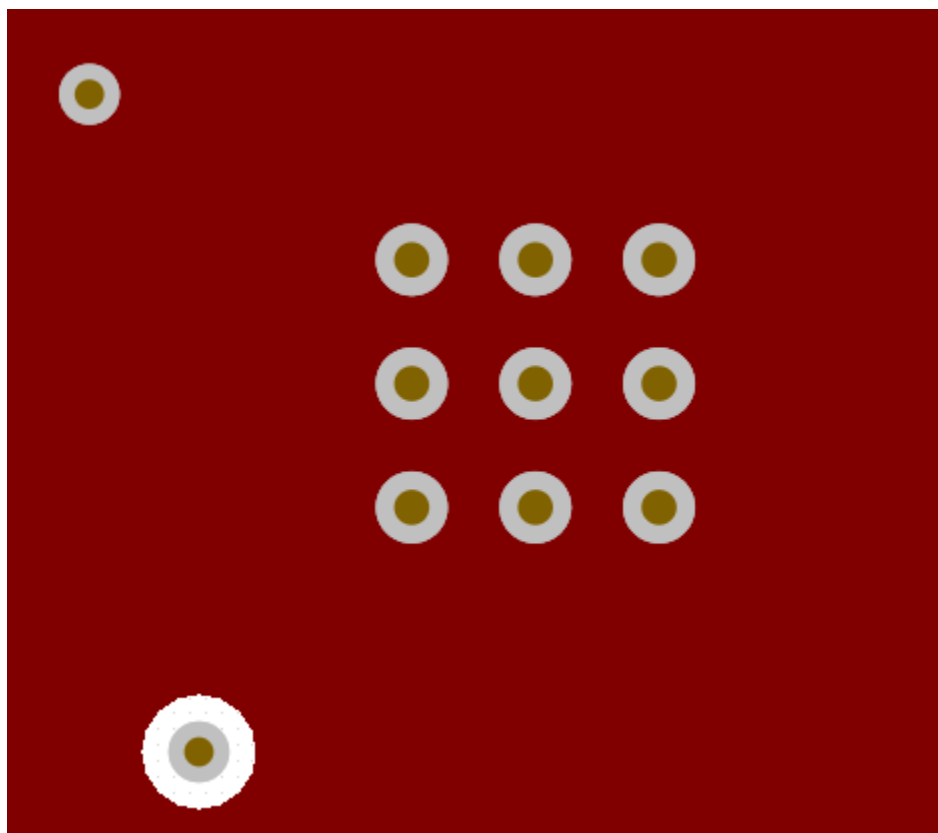
图 11-2. Recommended PCB Layout, GND Layer
