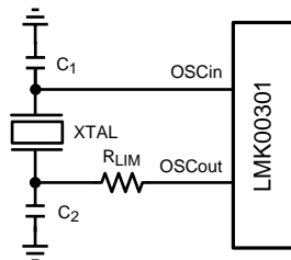
Figure 28. Crystal Interface
