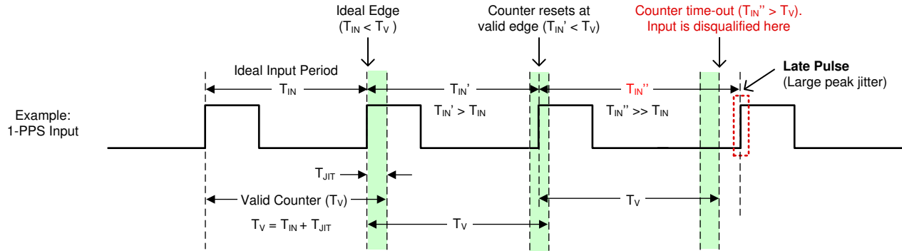
图 8-17. 1-PPS Input Window Detector Example
