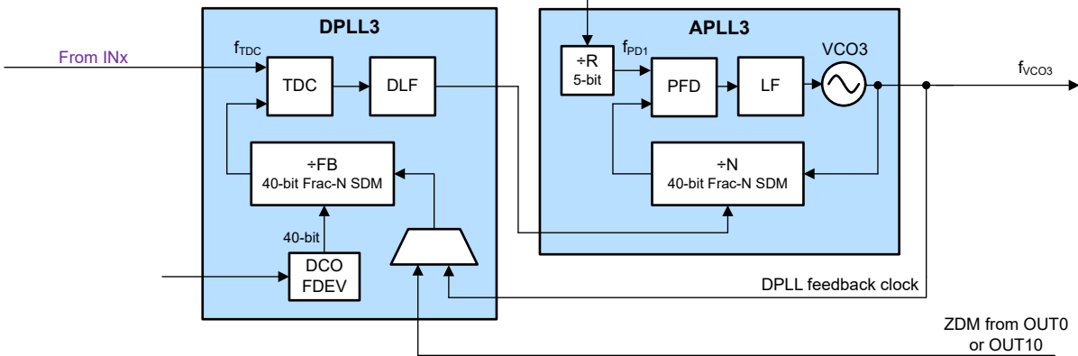
图 8-6. APLL Cascaded With DPLLs Disabled Example
