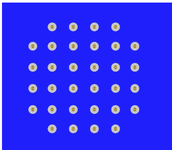
图 9-19. PCB Layout Example for LMK5B33216, Bottom Layer
