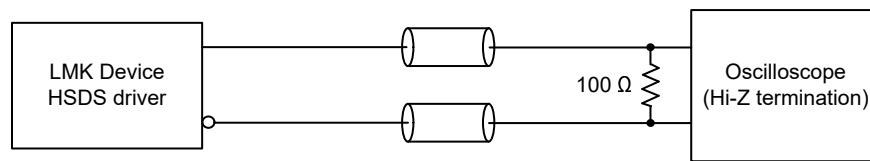
图 7-5. HSDS Output Time Domain Test Configuration
