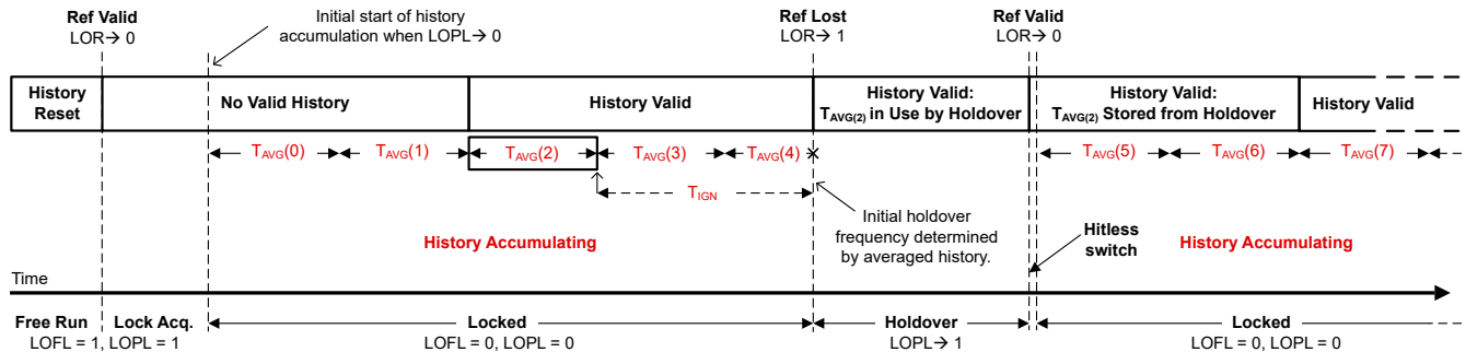
图 8-19. Tuning Word History Windows
