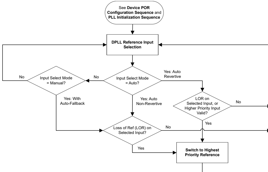
图 8-14. DPLL Reference Input Selection Flowchart
