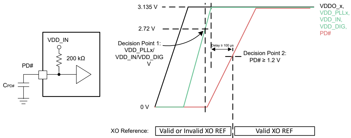
图 9-2. Recommendation for Power Up From Split-Supply Rails
