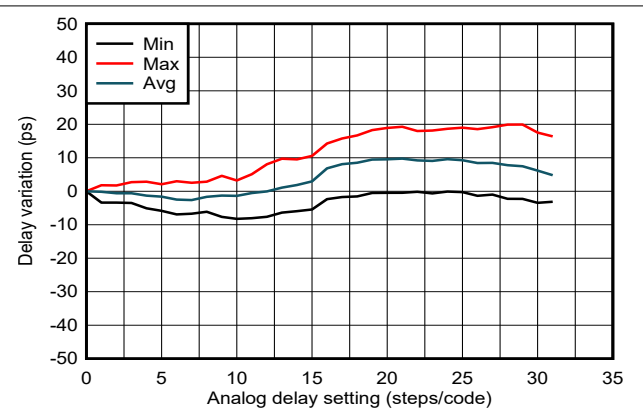
图 6-9. SYSREF/1-PPS Delay Linearity vs Analog Delay Code 3
