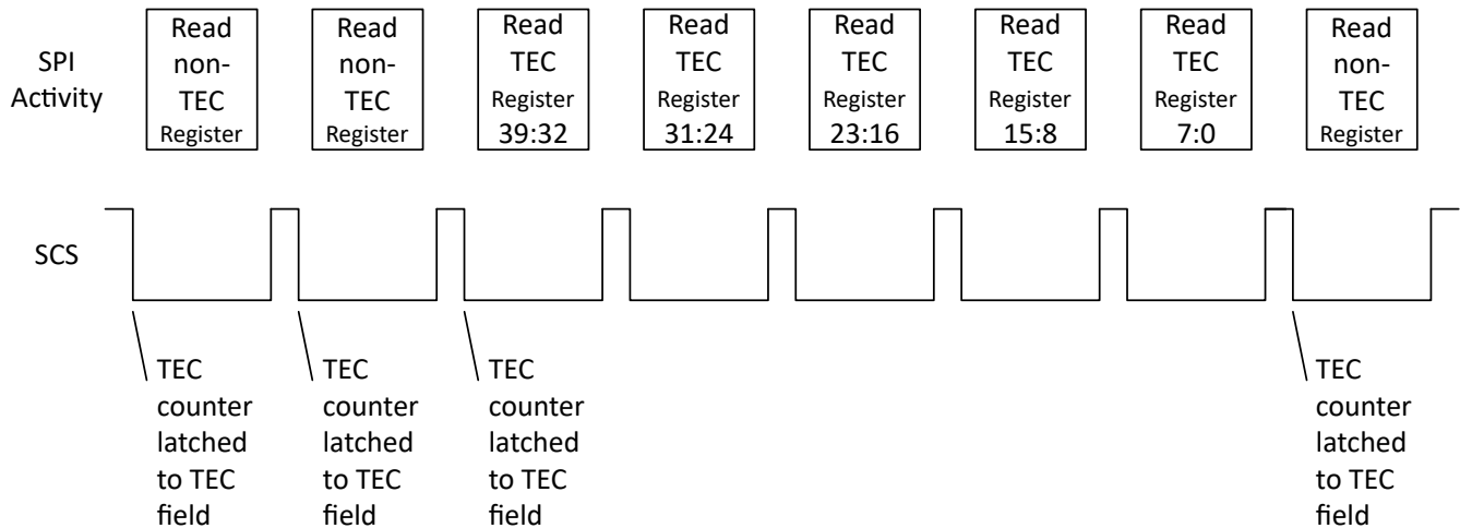
图 8-32. TEC Single Byte Read
