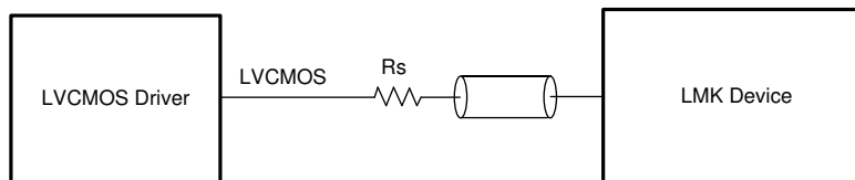
图 8-10. Single-Ended LVC MOS (1.8 V, 2.5 V, 3.3 V) to Reference (INx_P) or XO Input (XO)
