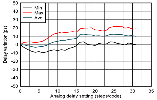
图 6-11. SYSREF/1-PPS Delay Linearity vs Analog Delay Code 5
