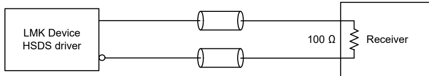
图 8-24. DC-Coupled HSDS Output Termination
