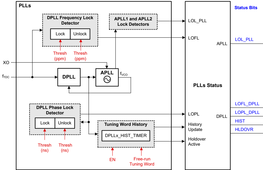
图 8-18. PLL Lock Detectors and History Monitor
