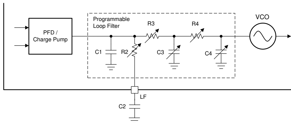
图 8-22. Loop Filter Structure of Each APLL
