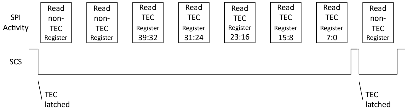
图 8-33. TEC Multibyte Read
