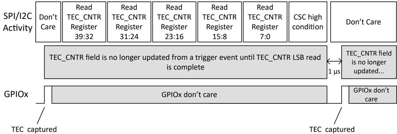
图 8-34. TEC Captured Using GPIO
