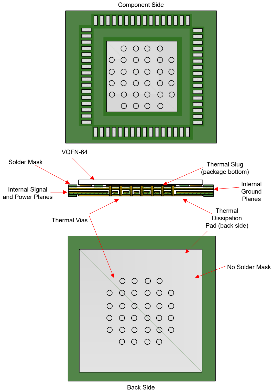
图 9-20. General PCB Ground Layout for Thermal Reliability (8+ Layers Recommended)
