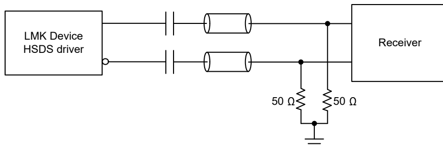
图 8-26. AC-Coupled HSDS Output Termination Method 2
