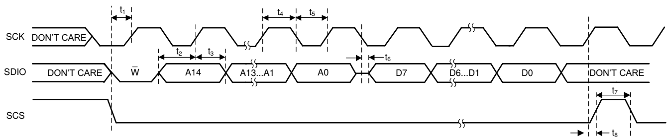
图 6-3. SPI 3-Wire Read Timing Diagram
