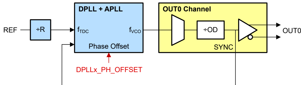
图 8-29. DPLL ZDM Synchronization Between Reference Input and OUT0
