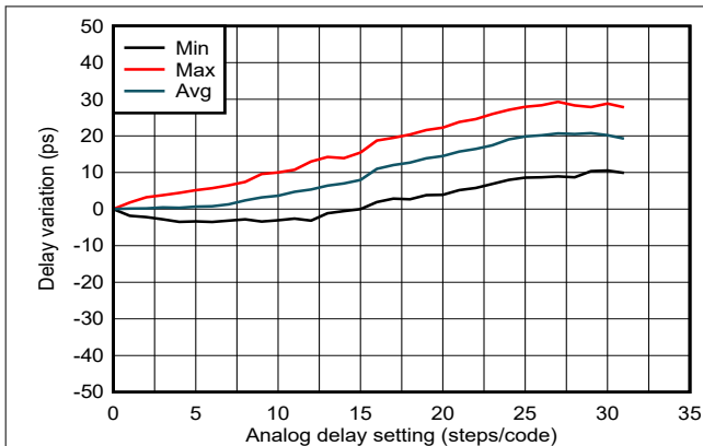
图 6-8. SYSREF/1-PPS Delay Linearity vs Analog Delay Code 2
