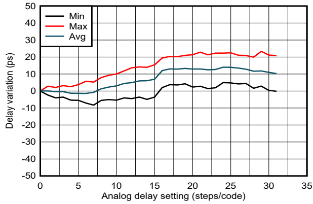
图 6-10. SYSREF/1-PPS Delay Linearity vs Analog Delay Code 4
