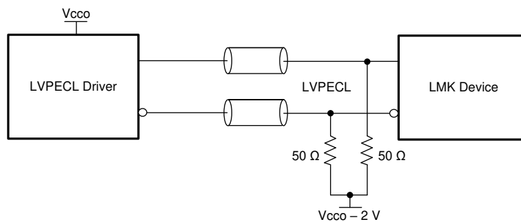
图 8-11. DC-Coupled LVPECL to Reference (INx)
