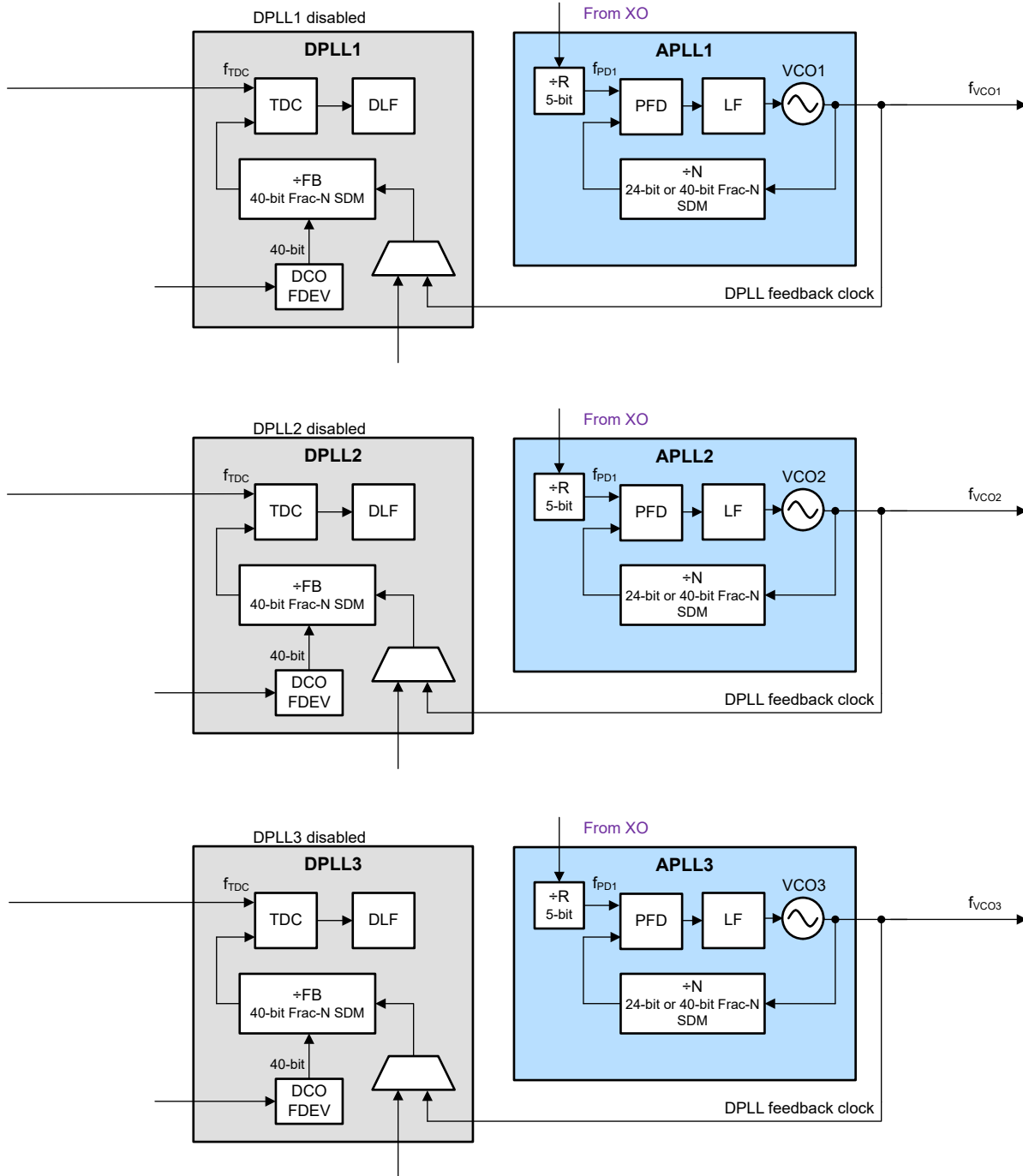
图 8-7. APLL-Only Independent Mode
