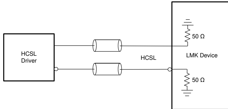
图 8-13. HCSL (Load Terminated) to Reference (INx)
