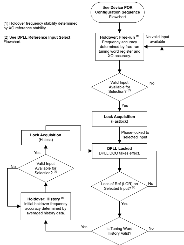
图 8-36. DPLL Operating States
