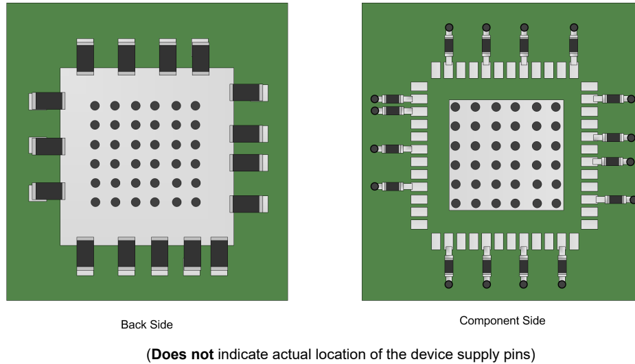
图 9-17. Generalized Placement of Power Supply Bypass Capacitors
