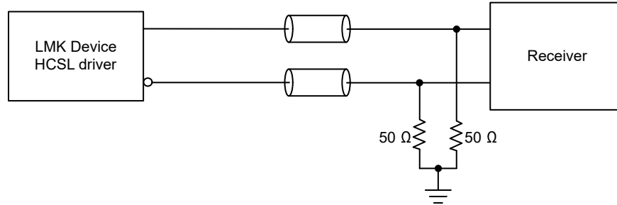
图 8-27. DC-Coupled HCSL Output Termination
