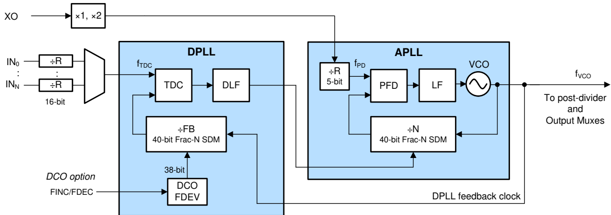
图 8-21. PLL Architecture
