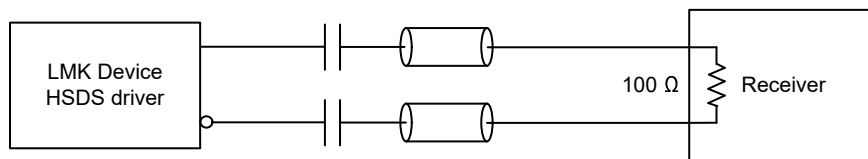
图 8-25. AC-Coupled HSDS Output Termination Method 1
