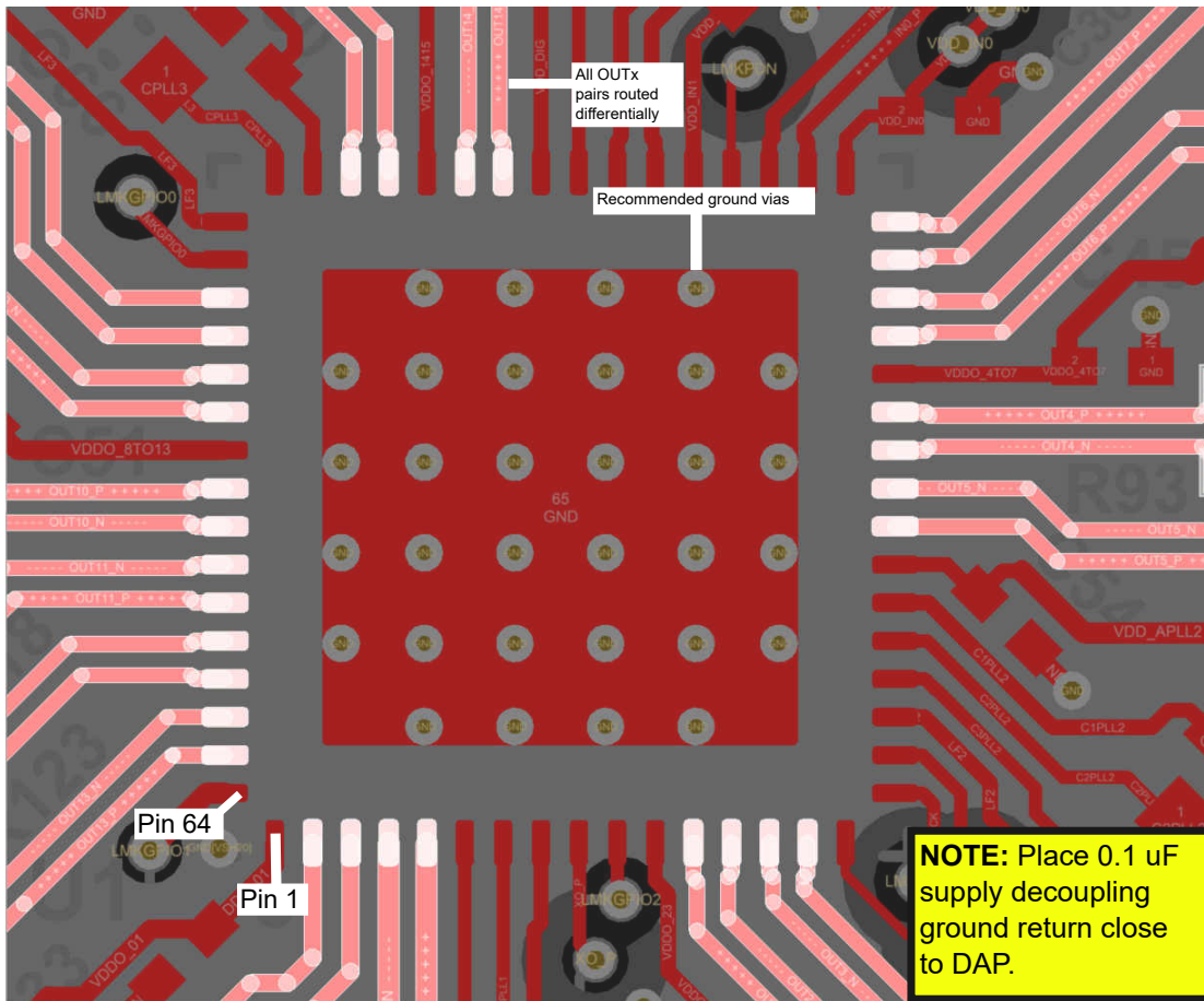
图 9-18. PCB Layout Example for LMK5B33216, Top Layer
