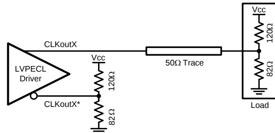
Figure 25. Single-Ended LVPECL Operation, DC Coupling, Thevenin Equivalent
