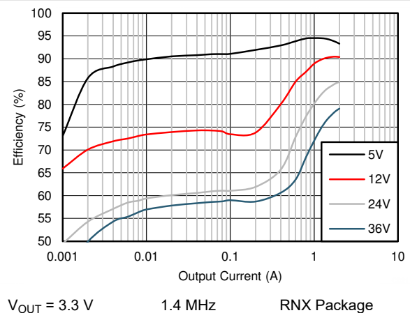
图 8-14. Efficiency
