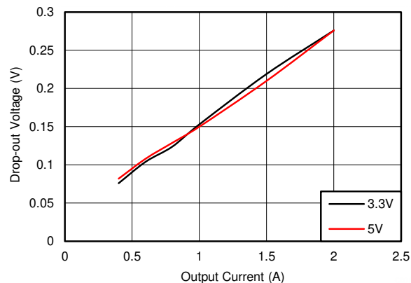
图 7-10. Typical Dropout Voltage versus Output Current in Frequency Foldback f_{SW} = 140\text{ kHz}
