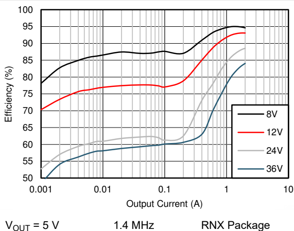
图 8-13. Efficiency
