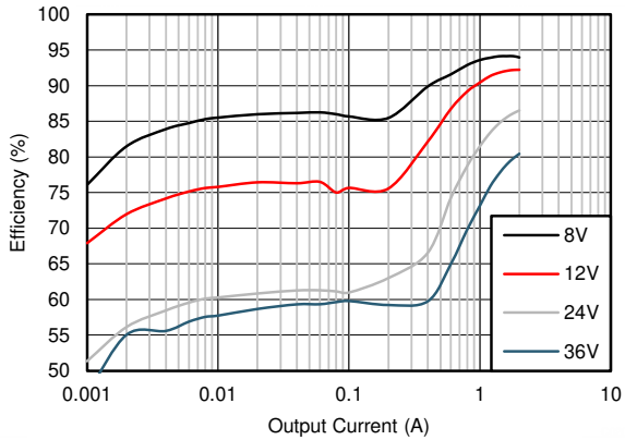
图 8-15. Efficiency
