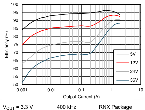
图 8-12. Efficiency
