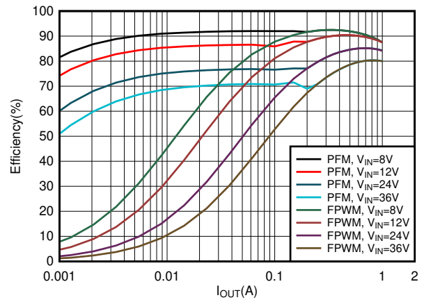
图 7-2. 5-V Efficiency versus Load Current
