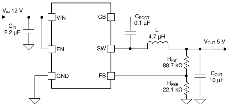
图 9-1. Application Circuit
