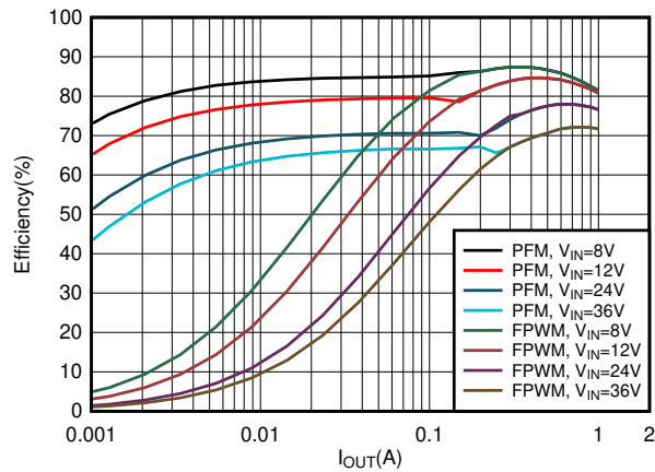
图 7-1. 3.3-V Efficiency versus Load Current
