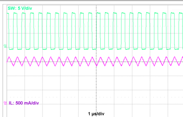
图 8-8. Typical PWM Switching Waveforms V_{IN} = 12 V, V_{OUT} = 5 V, I_{OUT} = 1.5 A, f_S = 2100 kHz
