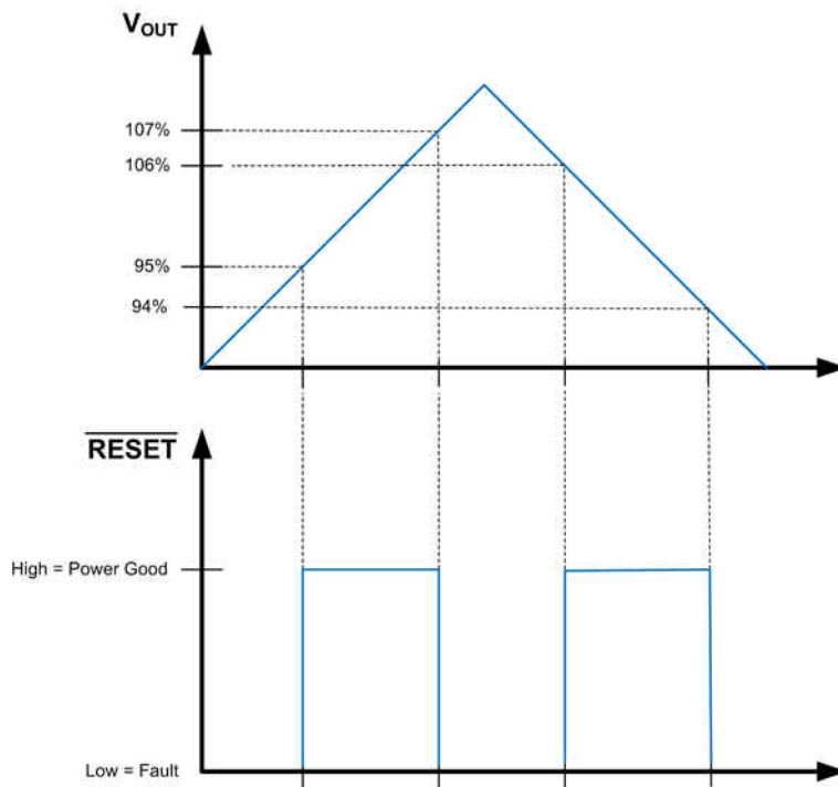
图 8-2. Static \overline{RESET} Operation
