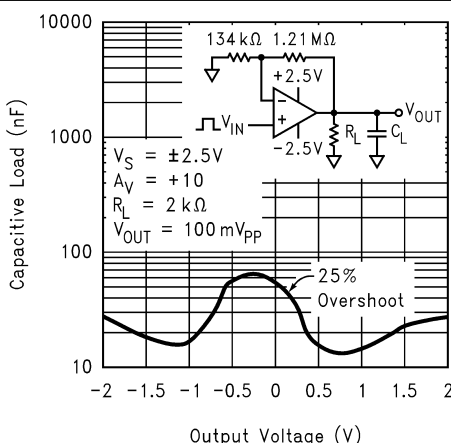
Figure 7-40. Stability vs Capacitive Load
