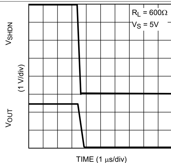
Figure 43. Turnoff Time
