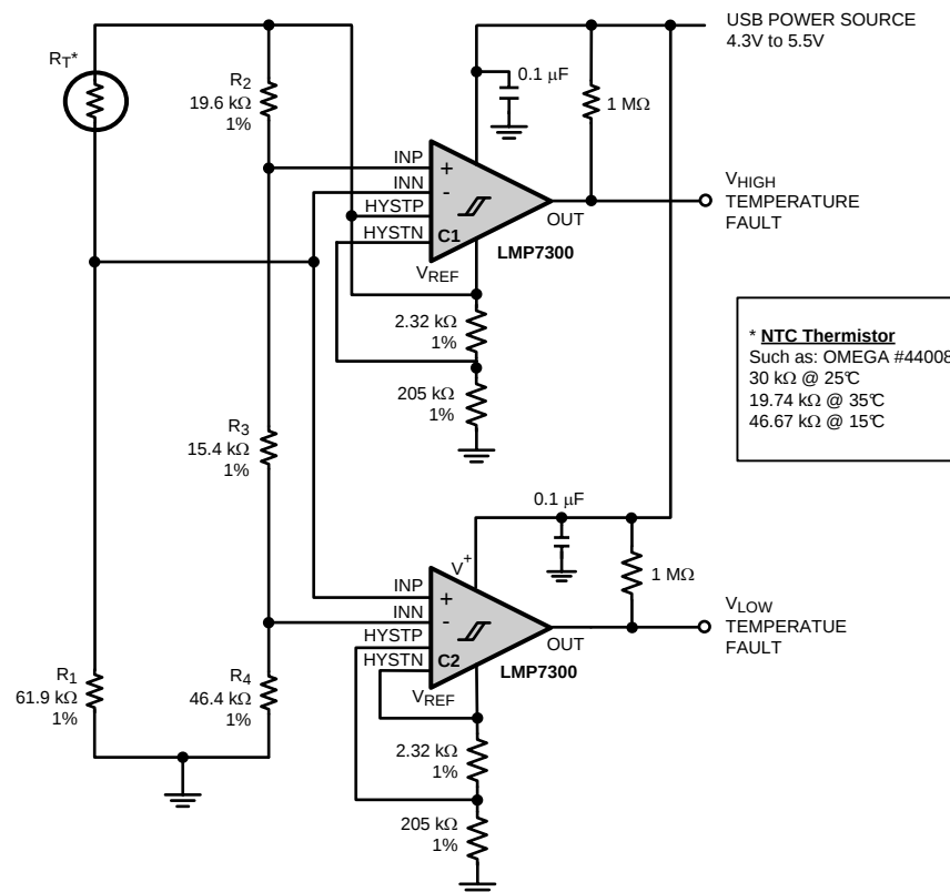
Figure 23. Temperature-Controlled Window Detector to Monitor Ambient Temperature
