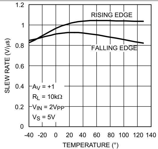
Figure 18. Slew Rate vs Temperature
