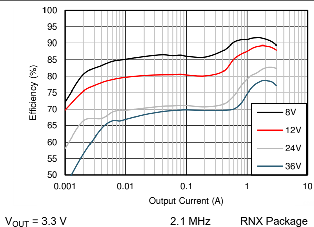
Figure 9-18. Efficiency
