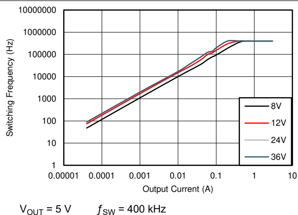
Figure 9-22. Switching Frequency versus Output Current
