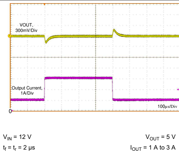
Figure 9-24. Load Transient
