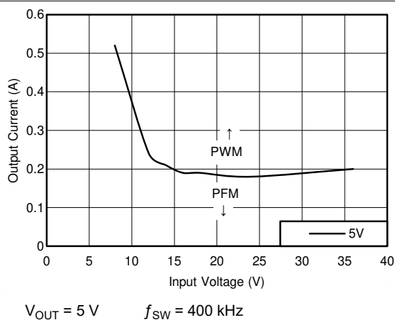
Figure 9-21. Mode Change Thresholds
