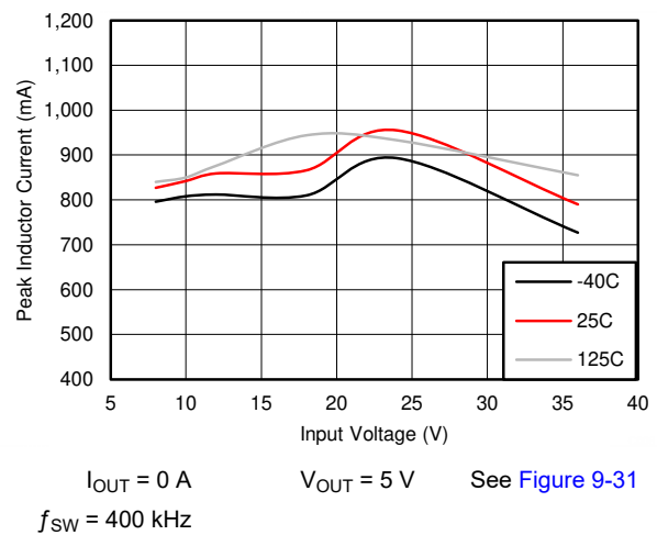
Figure 7-6. I_{PEAK-MIN}
