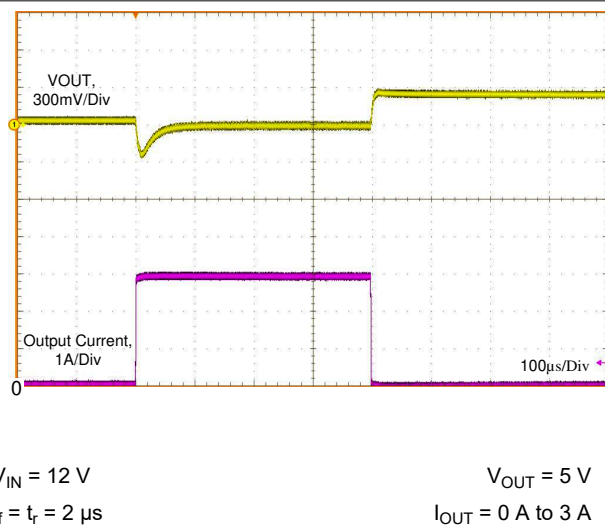
Figure 9-23. Load Transient
