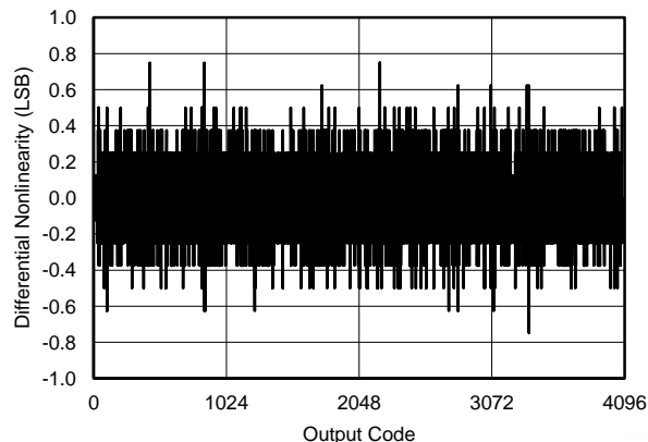
Figure 16. Differential Nonlinearity (Voltage Channel)
