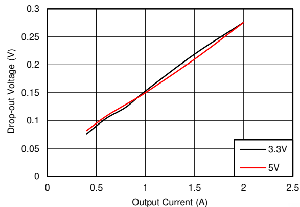
图 8-10. Typical Dropout Voltage versus Output Current in Frequency Foldback f_{SW} = 140\text{ kHz}
