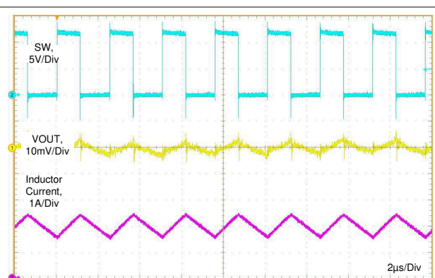
图 8-8. Typical PWM Switching Waveforms V_{IN} = 12 V, V_{OUT} = 5 V, I_{OUT} = 2 A, f_S = 400 kHz
