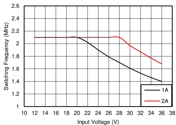
图 8-13. Switching Frequency versus Input Voltage V_{OUT} = 3.3\text{ V}
