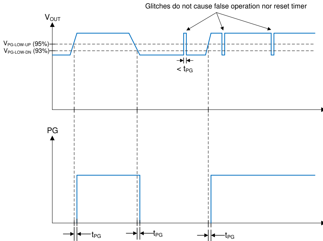
图 8-2. Power-Good-Timing Behavior
