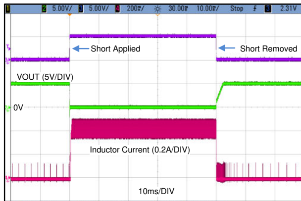
图 8-15. Short Circuit Waveform
