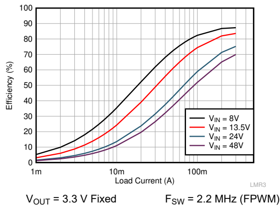
图 7-1. Efficiency 3.3-V Output, FPWM
