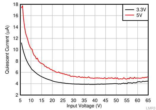
图 7-4. Typical Input Supply Current at No Load for Fixed 3.3-V and 5-V Output
