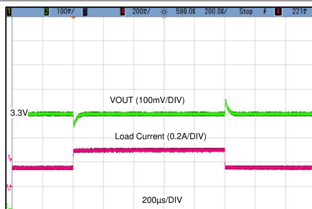
LMR36503MSC3 V_{OUT} = 3.3\text{ V} Fixed 2.2 MHz 0.15 A to 0.3 A, 1 A/μs
