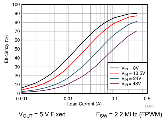
图 7-2. Efficiency 5-V Output, FPWM
