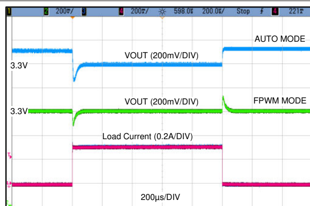
LMR36503MSC3 V_{OUT} = 3.3\text{ V} Fixed 2.2 MHz 0 A to 0.3 A, 1 A/μs
