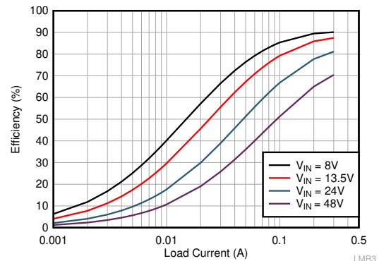
LMR36503MSC5 V_{OUT} = 5 V Fixed 2.2 MHz (FPWM)
