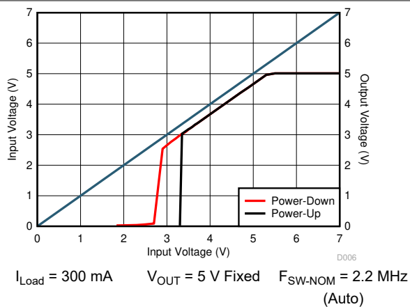
图 7-5. Dropout at Power-Up and Power-Down
