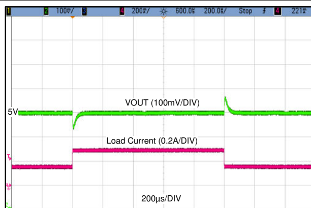
LMR36503MSC5 V_{OUT} = 5\text{ V} Fixed 2.2 MHz 0.15 A to 0.3 A, 1 A/μs
