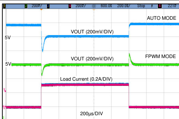
LMR36503MSC5 V_{OUT} = 5\text{ V} Fixed 2.2 MHz 0 A to 0.3 A, 1 A/μs
