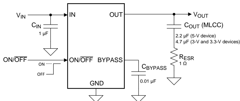
Figure 37. Typical Application With Ceramic C_{OUT} Series R
