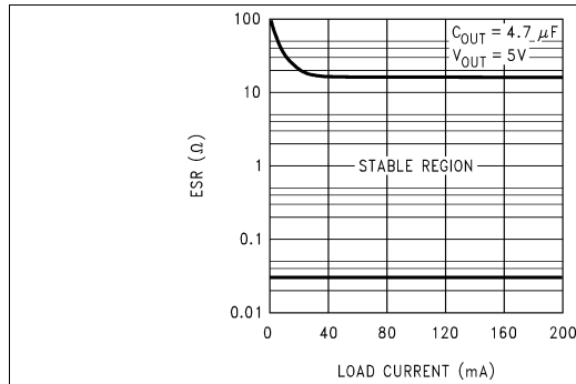
Figure 31. ESR Curves For 5-V Output
