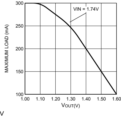
Figure 9. LDO Maximum Load
