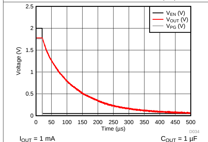
Figure 41. LP5912-1.8 V_{OUT} vs V_{EN(OFF)}
